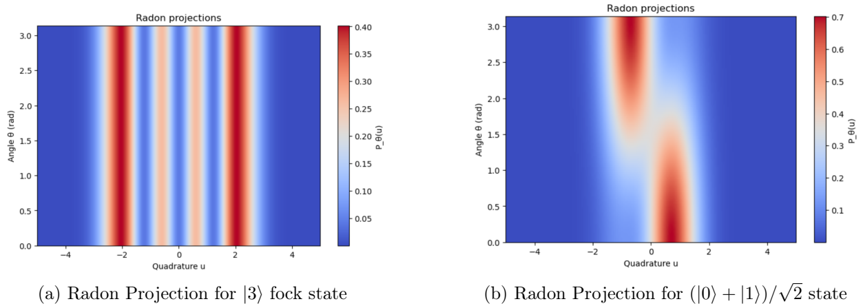
Figure 4: Radon Projections
